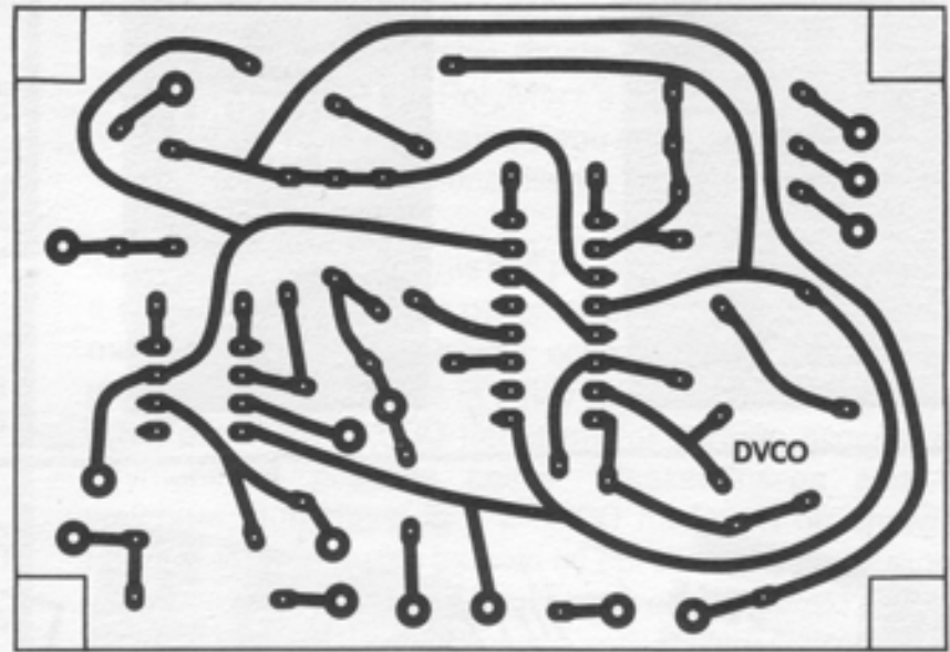
Foil Side
