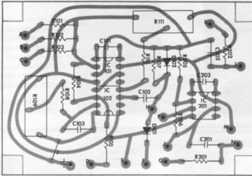
Component Side
